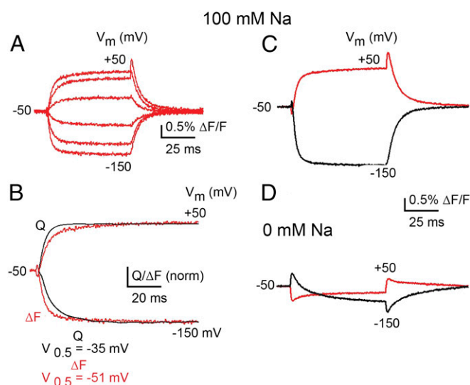
Fig. 5. Simultaneous recordings of voltage-induced charge movement (Q) and fluorescence ( \Delta F ) for SGLT1-T287C labeled with MTS-TAMRA. A single oocyte expressing SGLT1-T287C labeled with MTS-TAMRA was held at -50 mV, and changes in \Delta F were recorded in response to 100-ms step depolarizations (to +50 mV) and hyperpolarization (to -150 mV) in the presence of external \text{Na}^+ (100 mM NaCl). (A) Time course of the MTS-TAMRA \Delta F changes. (C) For clarity, only two \Delta F records are shown (at steps of +50 and -150 mV). (B) Time courses of simultaneous \Delta F and Q for voltage steps of +50 and -150 mV. The traces have been normalized (norm) to agree at the end of the voltage pulse (100 ms). The time constants ( \tau ) for the +50 mV pulse were 5 ms for Q and 10 and 75 ms for \Delta F , and for the -150 mV pulses, they were 5 ms for Q and 4.5 and 75 ms for \Delta F . (D) Time course of \Delta F for voltage jumps to +50 and -150 mV in the absence of \text{Na}^+ . Complete \Delta F and Q/V curves are given in SI Appendix , Fig. S2.
